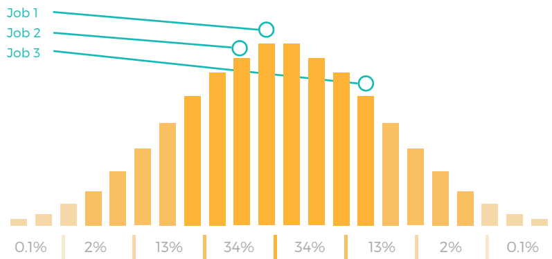
Distribution of COGNITIVE ABILITY
